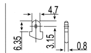
Terminal F1(187)
